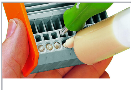
WAGO Rail-Mount Terminal Blocks (up to 4 mm 2 /12 AWG)
